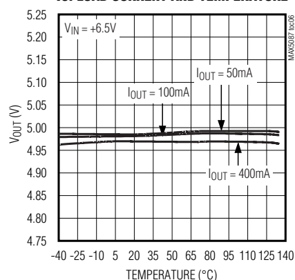
OUTPUT VOLTAGE vs. LOAD CURRENT AND TEMPERATURE
