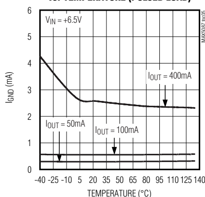
GROUND CURRENT vs. TEMPERATURE (PULSED LOAD)
